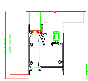
201 SILL SERIES 3000
